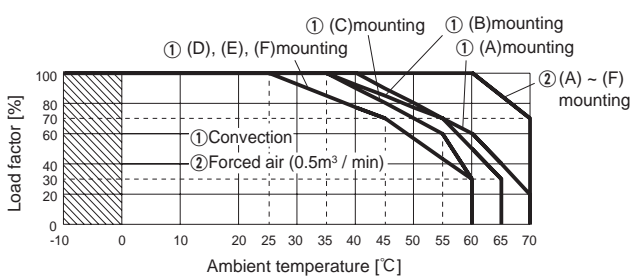
Fig.3.10 Ambient temperature derating curve (refer to Table 3.7)
