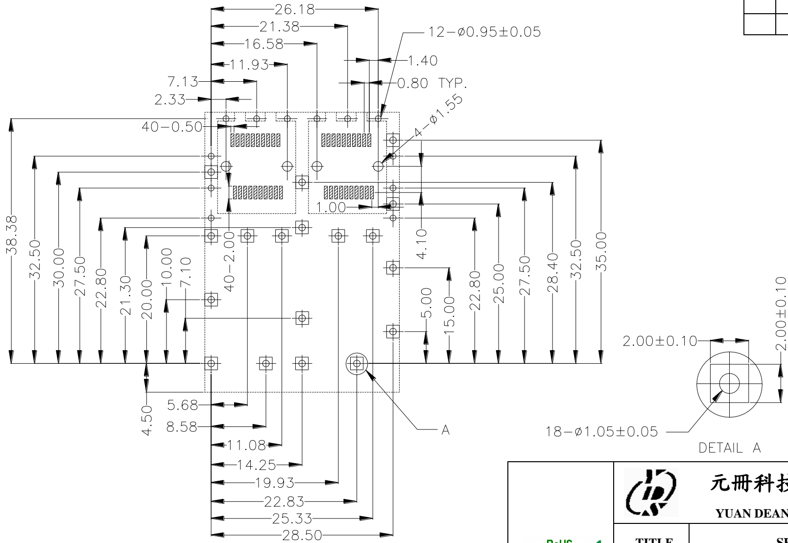
P.C.B. LAYOUT TOP VIEW ±0.05
